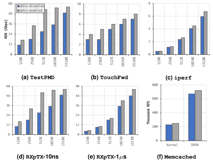
Fig. 14. Effect of Direct Cache Access (DCA) on Maximum Sustainable Bandwidth (MSB) when running TestPMD TouchFwd, iperf, RXP-TX (with 10ns & 1µs processing time), MemcachedDPDK, & MemcachedKernel on gem5.
