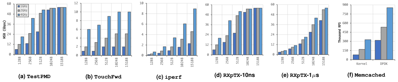
Fig. 15. Effect of Core Frequency on Maximum Sustainable Bandwidth (MSB) when running TestPMD TouchFwd, iperf, RXpTX (with 10ns & 1µs processing time), MemcachedDPDK, & MemcachedKernel on gem5.
