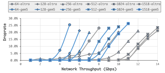
Fig. 7. Comparing the bandwidth vs. drop rate for TouchFwd on gem5 and real system (altra configuration). The number in the legend show the packet size in bytes.
