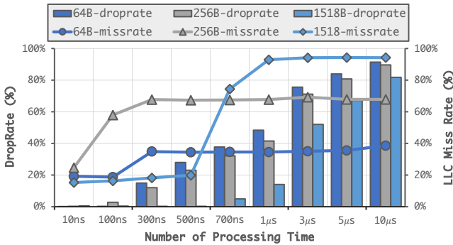
Fig. 13. Effect of the performance of various policies for DCA using 64B, 256B, and 1518B packets when running RXP-TX with processing time set to 10ns, 100ns, 300ns, 500ns, 700ns, 1µs, 3µs, 5µs 10µs with ring buffer size set to 4096.
